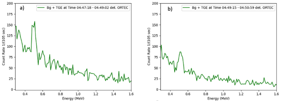
Figure 5. NGR spectrograms obtained with the ORTEC spectrometer during positive a) and negative b) NSEF, as indicated by lines in Figure 4.
