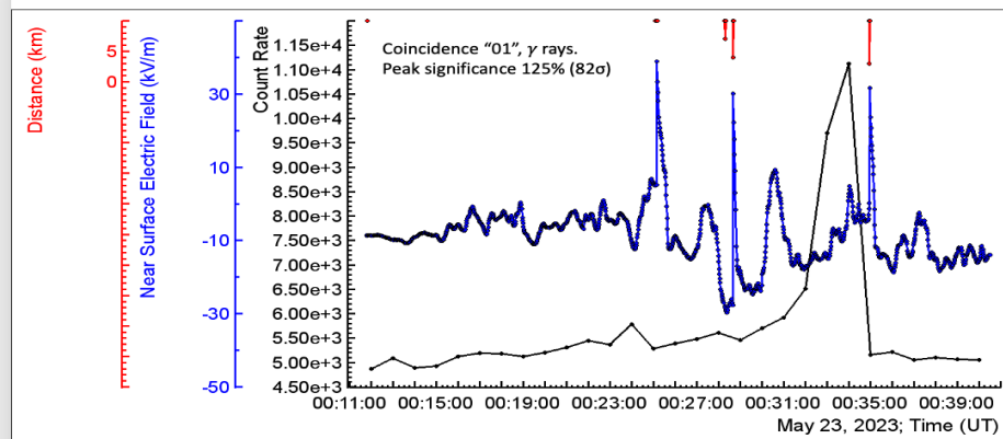
Figure 14. One minute time series of the “01” coincidence measured by CUBE detector on Aragats, black; One second time series of NSEF, blue, and distances to lightning flash, red.
