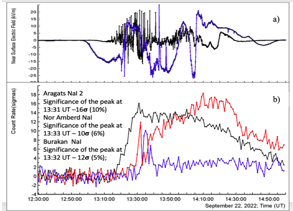
Figure 12. a) Disturbances of the NSEF measured on Aragats (black) and in Nor Amberd (blue); b) 1-minute time series of count rates of NaI (Tl) detectors on Aragats (black), in Nor Amberd (blue), and in Burakan (red).
